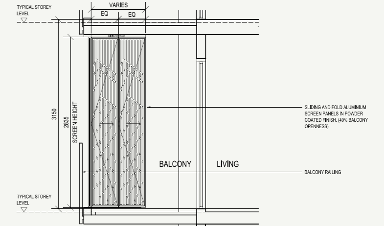
2 BALCONY / PES SCREEN - SECTION A-A (Internal View)
