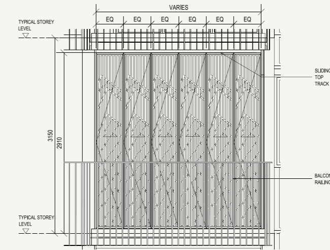
3 BALCONY / PES SCREEN - FRONT ELEVATION (External View)
